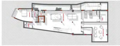
PRELIMINARY LOWER GROUND FLOOR
