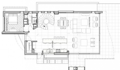
PRELIMINARY GROUND FLOOR
